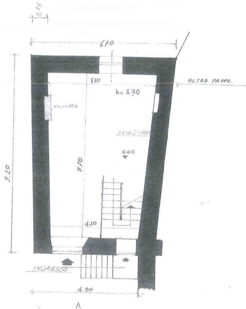
PIANO TERRA
